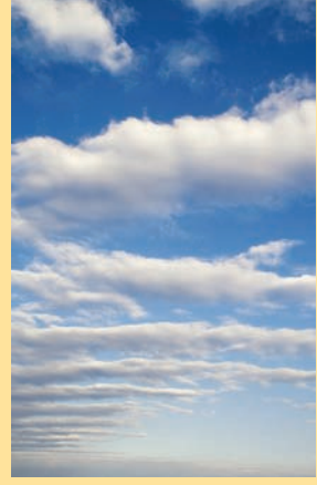
clouds
