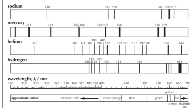
Absorption spectra
