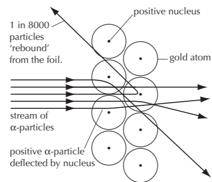
NB not to scale. Only a minute percentage of alpha-particles are scattered or rebound.
