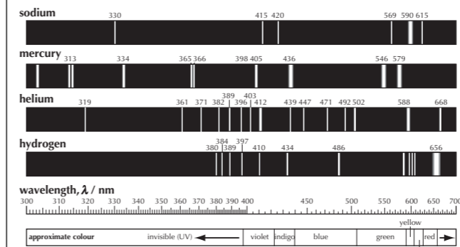
Emission spectra
