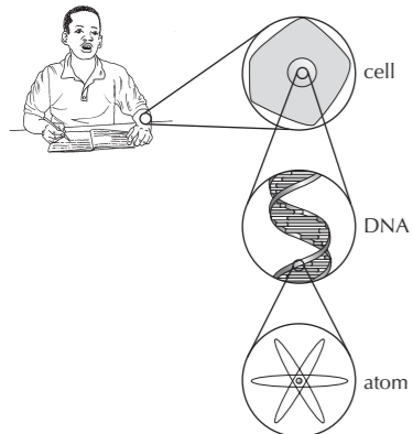
In the basic atomic model, we are made up of protons, neutrons, and electrons – nothing more.
